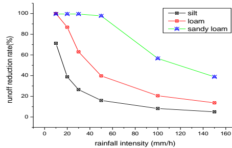
Figure 4. Soil types vs. Runoff Reduction Rate
