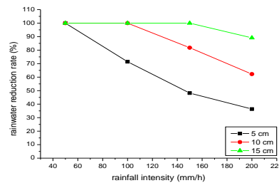
Figure 5. Concave Depth vs. Runoff Reduction Rate
