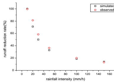
Figure 3. Rainfall intensity vs. Runoff Reduction Rate
