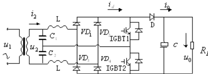
Figure 6. The Boost Chopper Improved
