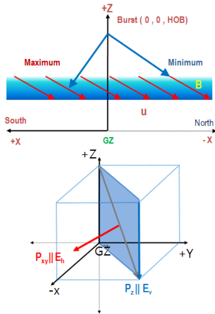
Figure 4. Wave polarization and unit vector
