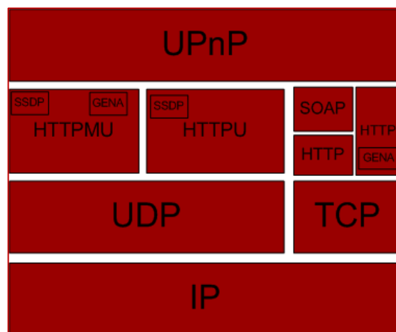
Figure 1. UPnP Stack.
