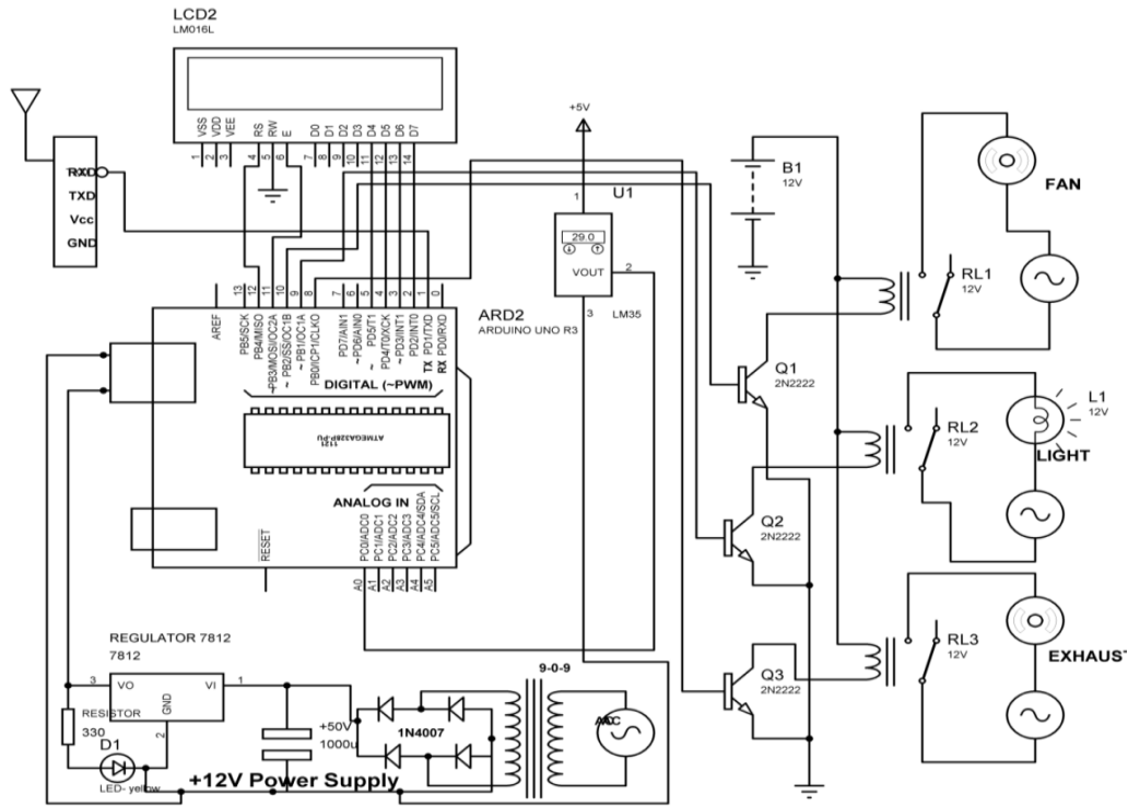
Figure 4. Circuit Diagram for Receiving Unit
