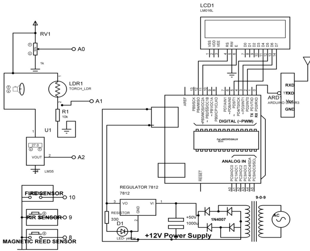
Figure 3. Circuit Diagram for Sensing Unit
