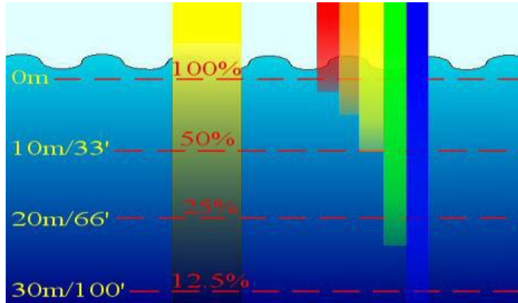
Figure 6. Absorption of light by water
