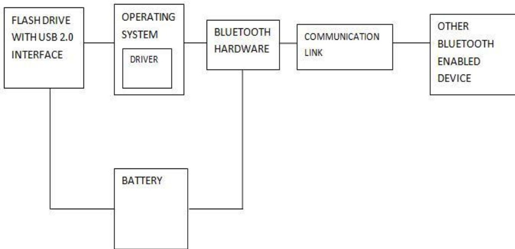
Figure 9. Proposed Block Diagram Bluetooth in USB
