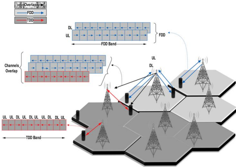
Figure 2. Two Overlapped LTE Cells (LTE-TDD with LTE-FDD)
