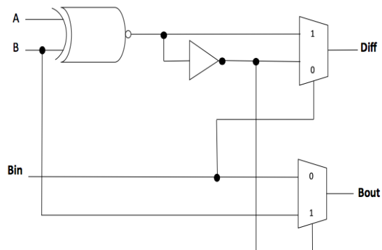
Figure 5(b). XNOR based Full Subtractor-2
