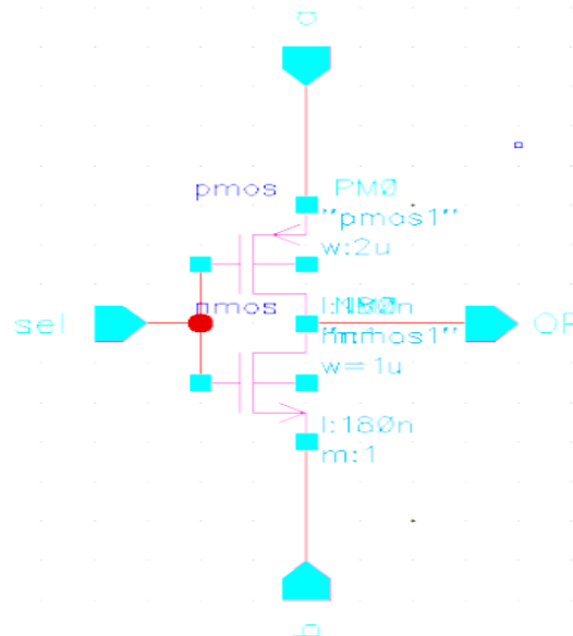
Figure 7. Multiplexer Design
