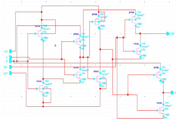
Figure 9(c). Schematic of XNOR based Full Subtractor-2
