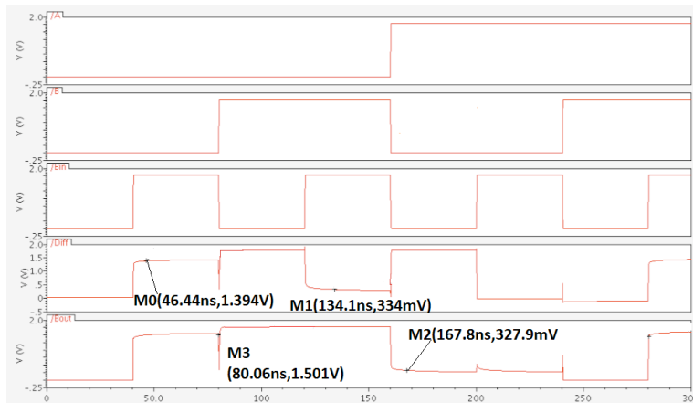
Figure 9(b). Output of XNOR based Full Subtractor-1
