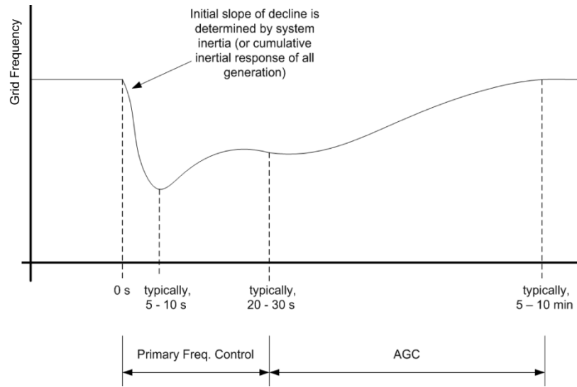
Figure 6. Inertial, Primary Frequency Controls, and AGC (Secondary) Response (Figure Courtesy Pouyan Pourbeik of EPRI)
