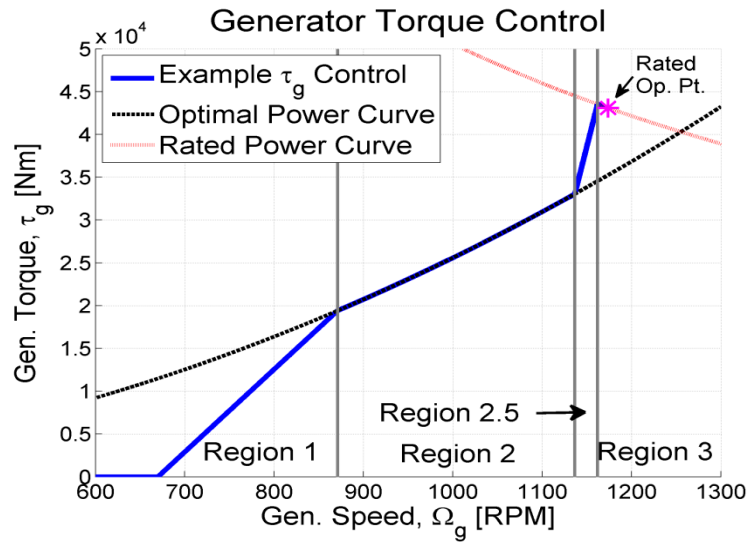
Figure 4. An Example of the Generator Torque Control in Different Operating Regions, as Described in [8]
