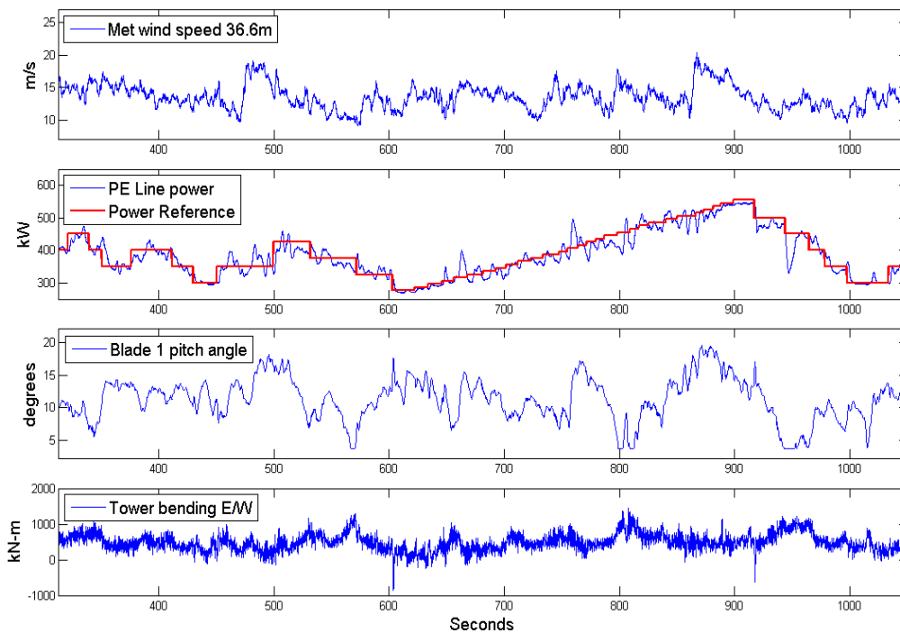
Figure 10. Field Test Data of Power Reference Tracking on CART3 Shows that sudden changes in the Power Reference Induce Increased Tower Bending Moment
