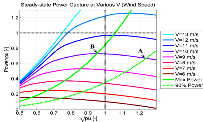
Figure 9. Various Steady-State Power Capture Curves for Given Wind Speeds
