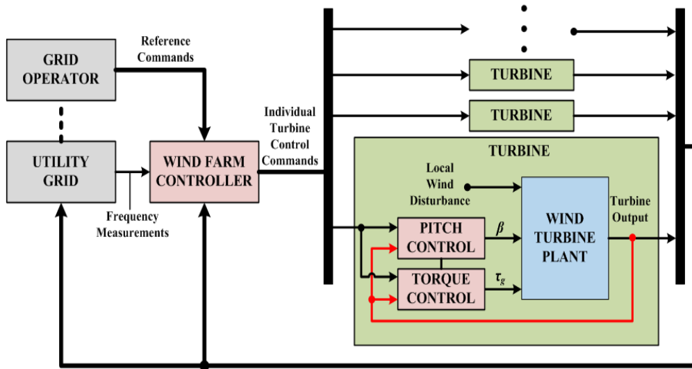
Figure 7. A Block Diagram that Shows the General Interconnection for APC Commands
