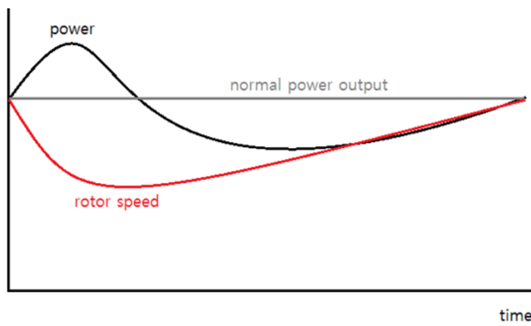
Figure 8. Inertial Response Emulation showing Sudden Electrical Power Increase with a Long Recovery Period
