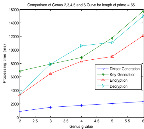
Figure 1. Genus g Vs processing time for length of prime = 65
