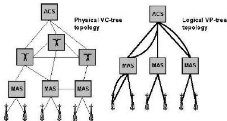
Figure 4. MN" A VP Topology
