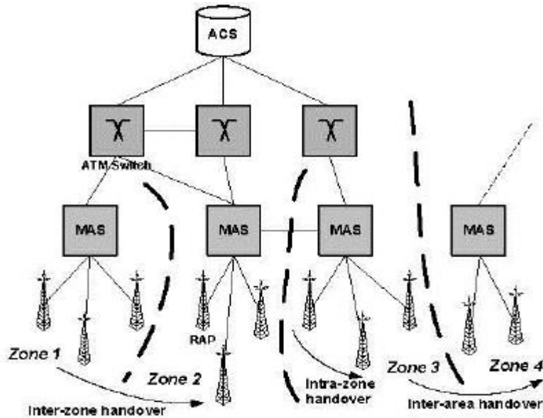
Figure 1. Architecture of the Wireless ATM Network
