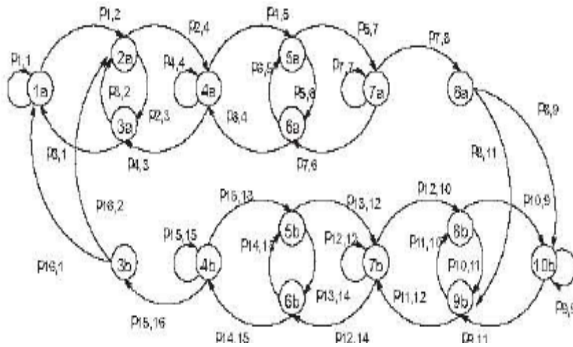
Figure 10. Discrete Markov Model for the Handover Succession with Hysteresis
