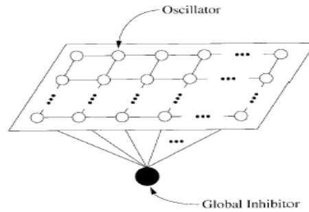
Figure 1: A 2-D LEGION network with four-neighborhood connections.
