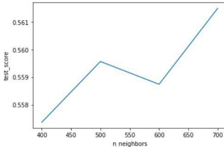
Figure 4. Graph plotting KNN score vs Neighbors
