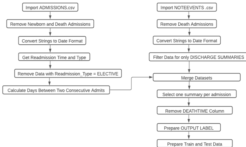
Figure 1. Prepare data
